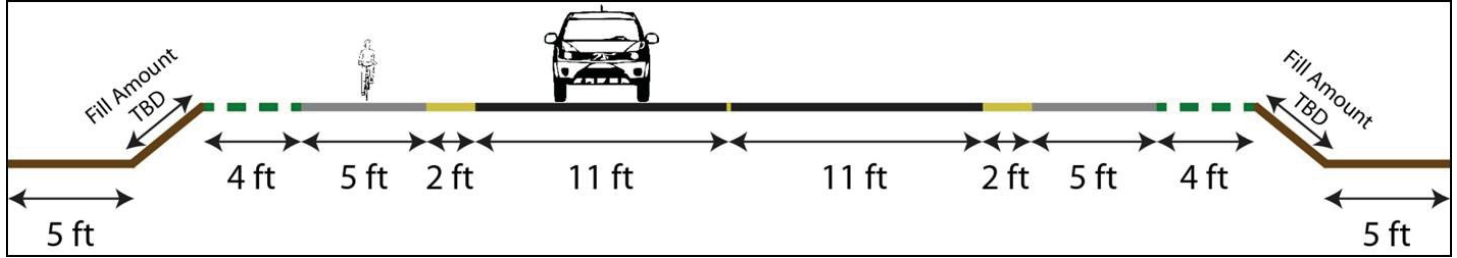
Proposed Bike and Pedestrian Use Enhancements Project at Davis Bayou, Mississippi District, Gulf Islands National Seashore, cross-section of typical roadway improvement
